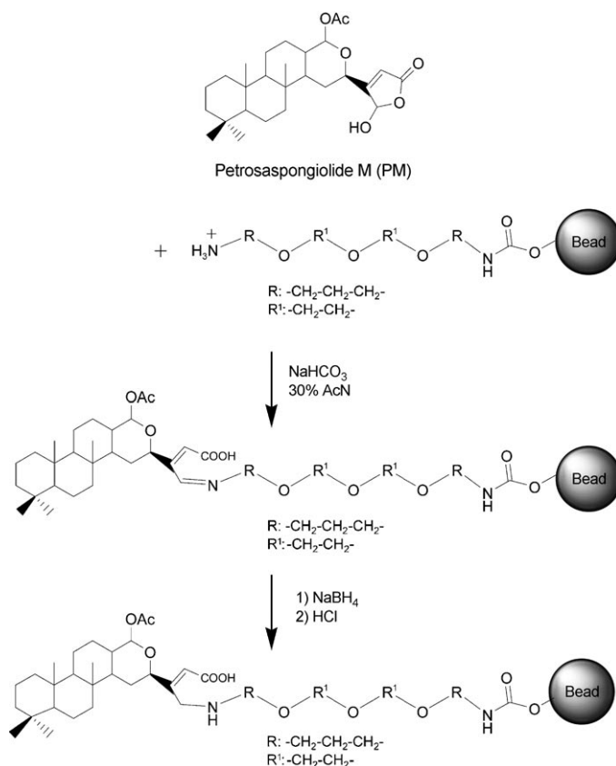
Scheme 1. Chemical structure of petrosapongiolide M (PM) and preparation of PM-modified beads.
